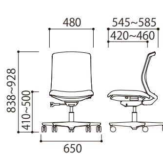
Middle Back Without Armrest
